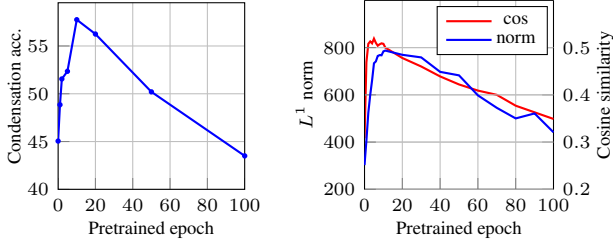
Figure 5. (Left) Condensation performance from fixed pretrained networks. The x-axis represents the number of epochs a network is trained on. (Right) Gradient analysis of the pretrained networks. The left axis measures the L^1 norm of the network gradients given a batch of data consisting of the same class. The right axis measures the average pairwise cosine-similarity between the gradients on a single data of the same class. The values are measured on ImageNet with 10 subclasses.
